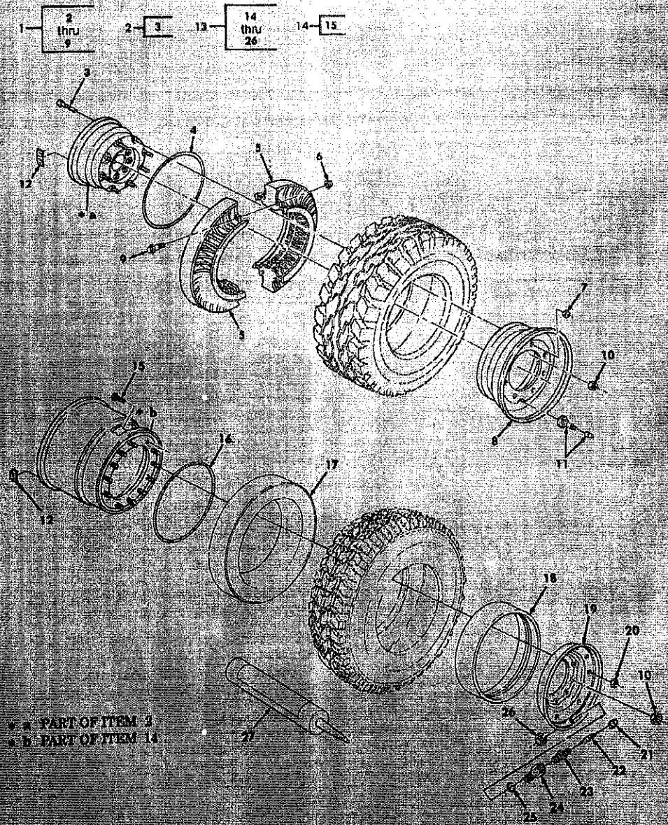
Figure 107. Wheel and Runflat Assembly
